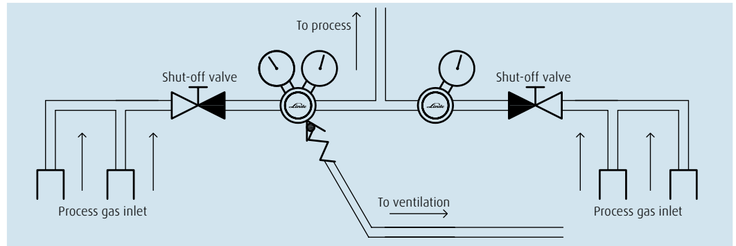
A 107 C4 with inlet shut-off valves
