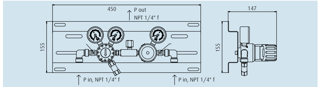
A 107 C2 with inlet check valves
