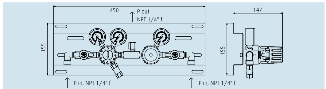
A 107 C2 with inlet shut-off valves
