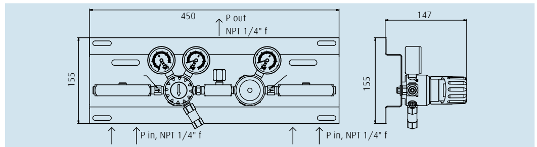
A 107 C4 with inlet check valves
