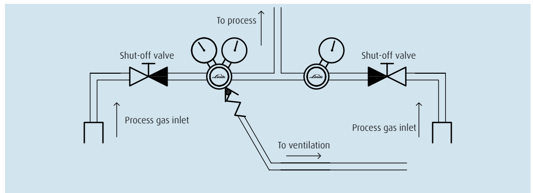
A 107 C2 with inlet shut-off valves
