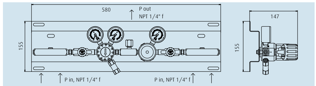
A 107 C4 with inlet shut-off valves
