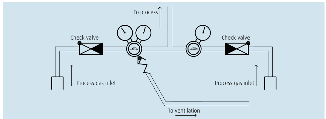
A 107 C2 with inlet check valves
