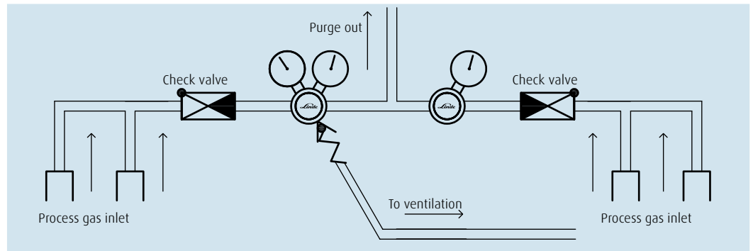
A 107 C4 with inlet check valves
