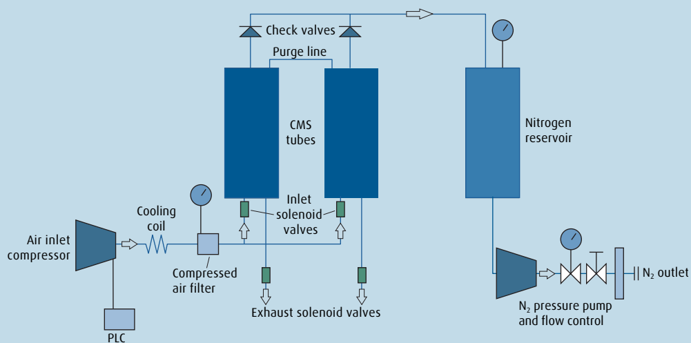
HiQ® LC/MS Plus nitrogen generator in principal.
