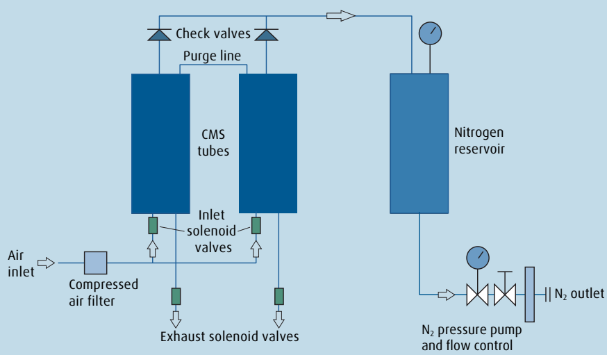
HiQ® ELSD nitrogen generator in principal.
